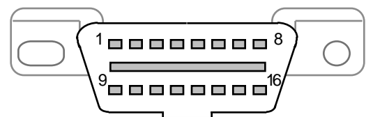
Figure 1. Vehicle Connector
